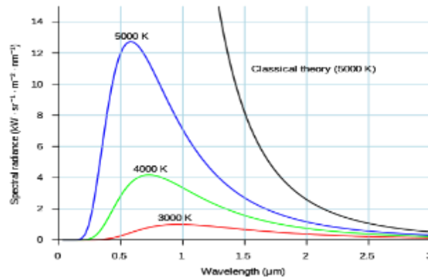
A1.8 - Blackbody radiation
