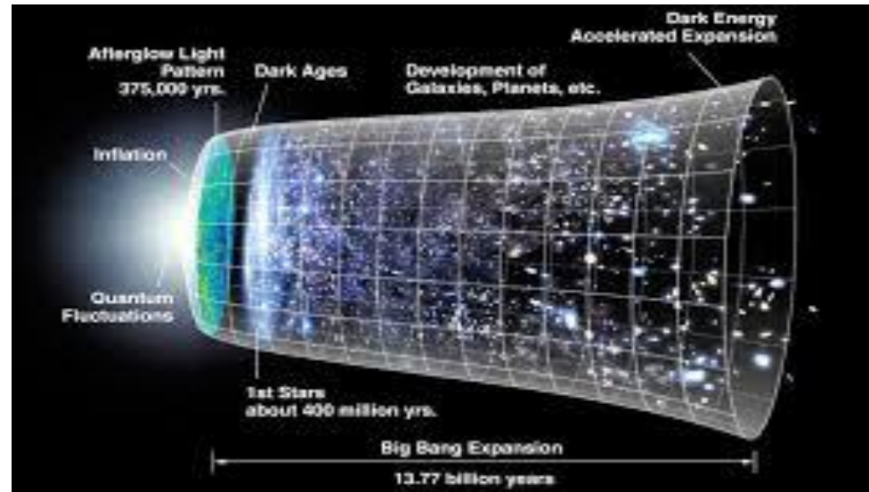
A1.7- Schematic representation of Big Bang and the expansion of the universe
