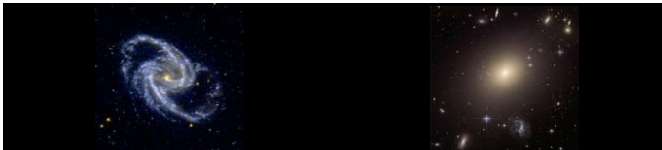
A1.10- A Spiral galaxy
