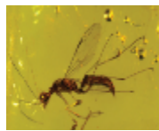
A2.26 - Cenozoic - Miocene (26-12 m)
