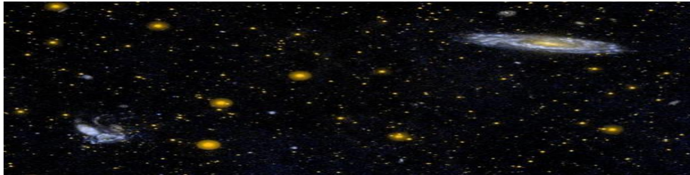
A1.5 - Galaxy cluster
