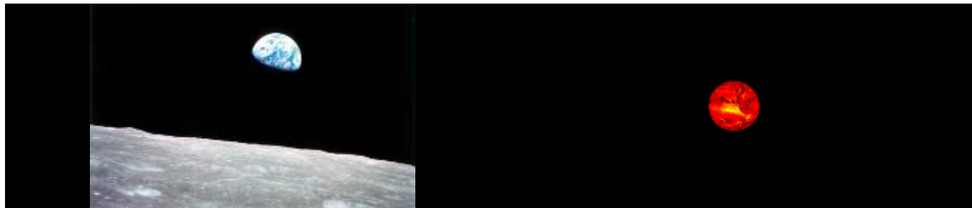
A6.5 - Earth seen from the moon
